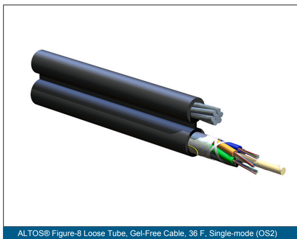
ALTOS® Figure-8 Loose Tube, Gel-Free Cable, 36 F, Single-mode (OS2)
