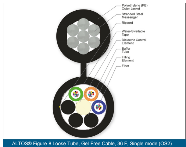
ALTOS® Figure-8 Loose Tube, Gel-Free Cable, 36 F, Single-mode (OS2)
